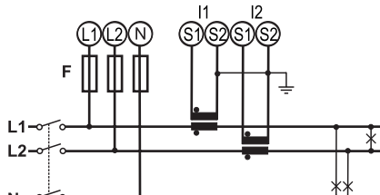
Fig. 15 Two-phase system (3-wire), 2 CT. 315 mA fuse (F).
