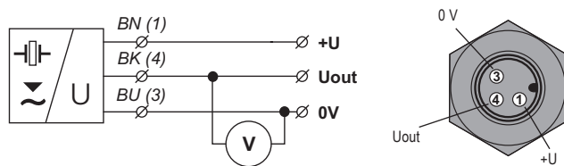
Connection diagram of the ULM level meter (variant -U) and inside view of the connector
