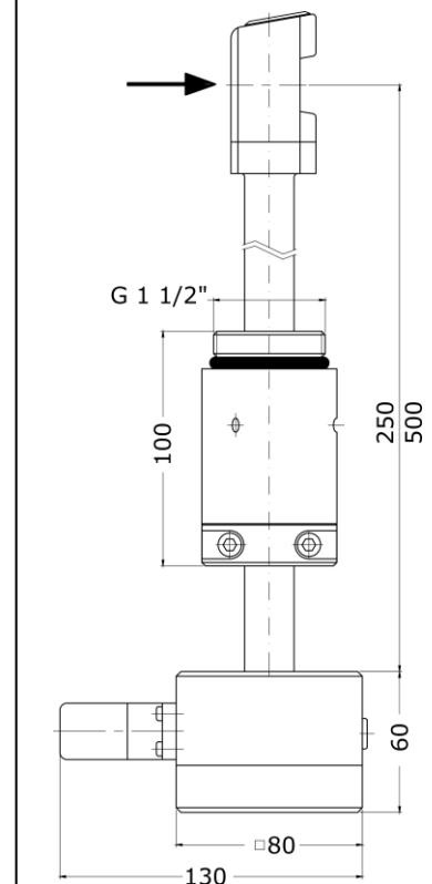
Vortex Flow Sensor VA40
