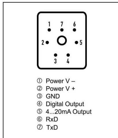
pin configuration plug GO 070
