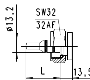
Sensor with union nut for T-piece G 3/8..G 1/2 Type ..031.. (L = 31 mm) or T-piece G 3/4..G 2 Type ..037.. (L = 37 mm)
